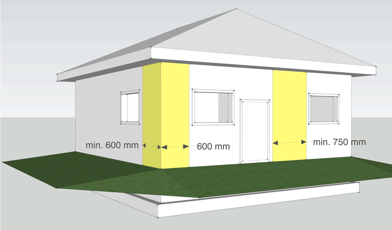
Minimum length of braced wall panels when connecting to intersecting braced wall panels, and minimum panel length in the field of the wall. xi
