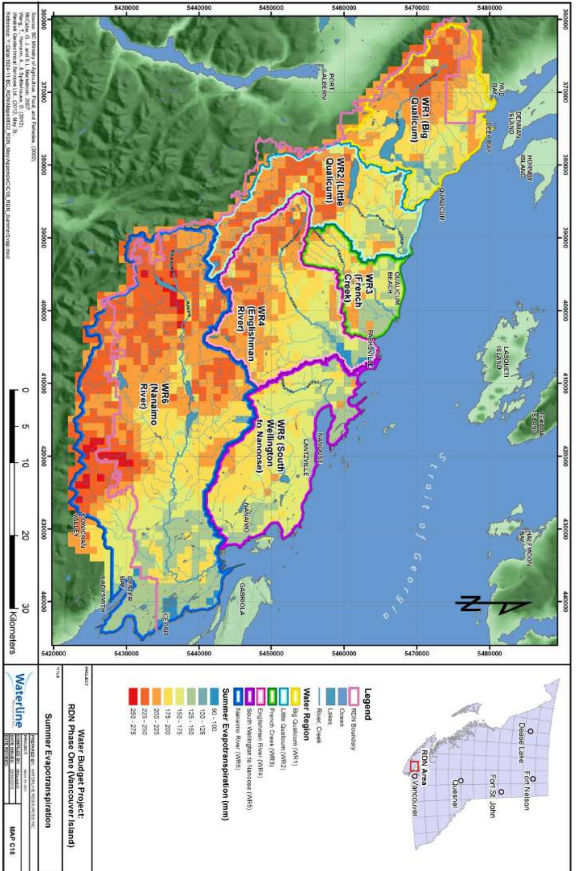
Map C18: Summer Evapo-transpiration See map C13 for description.
