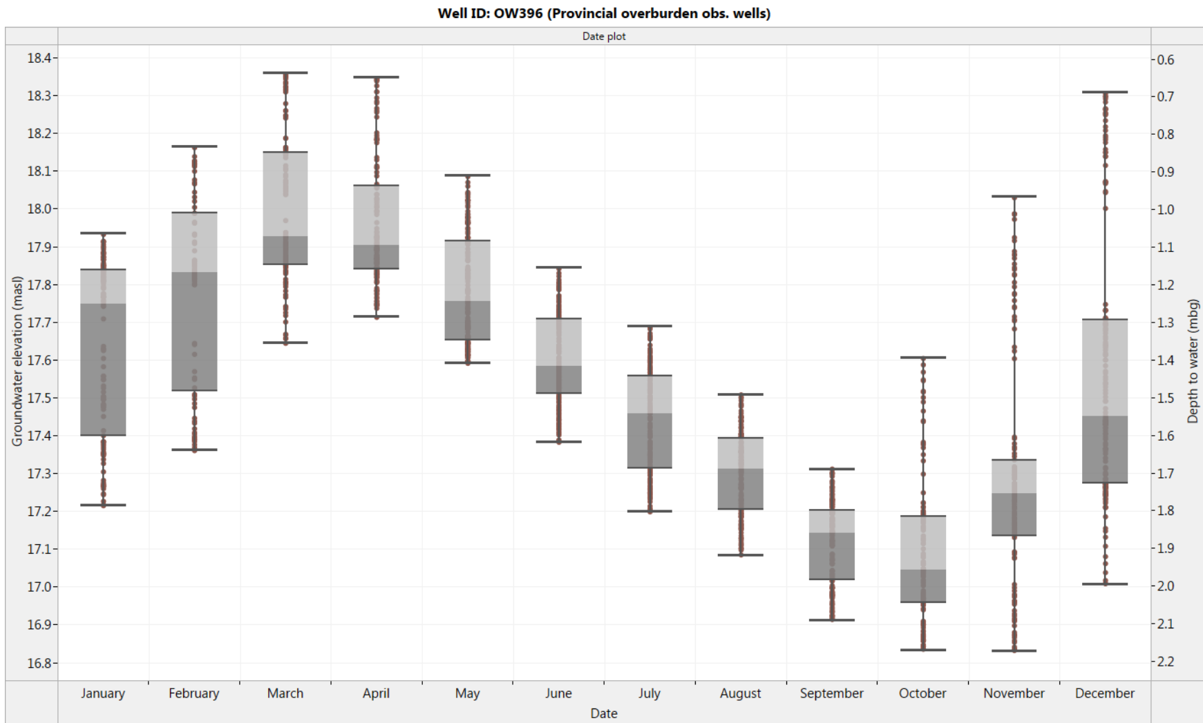
Figure 11. OW396: Box and Whisker diagram for historical monthly groundwater level fluctuation (2012-2016)
