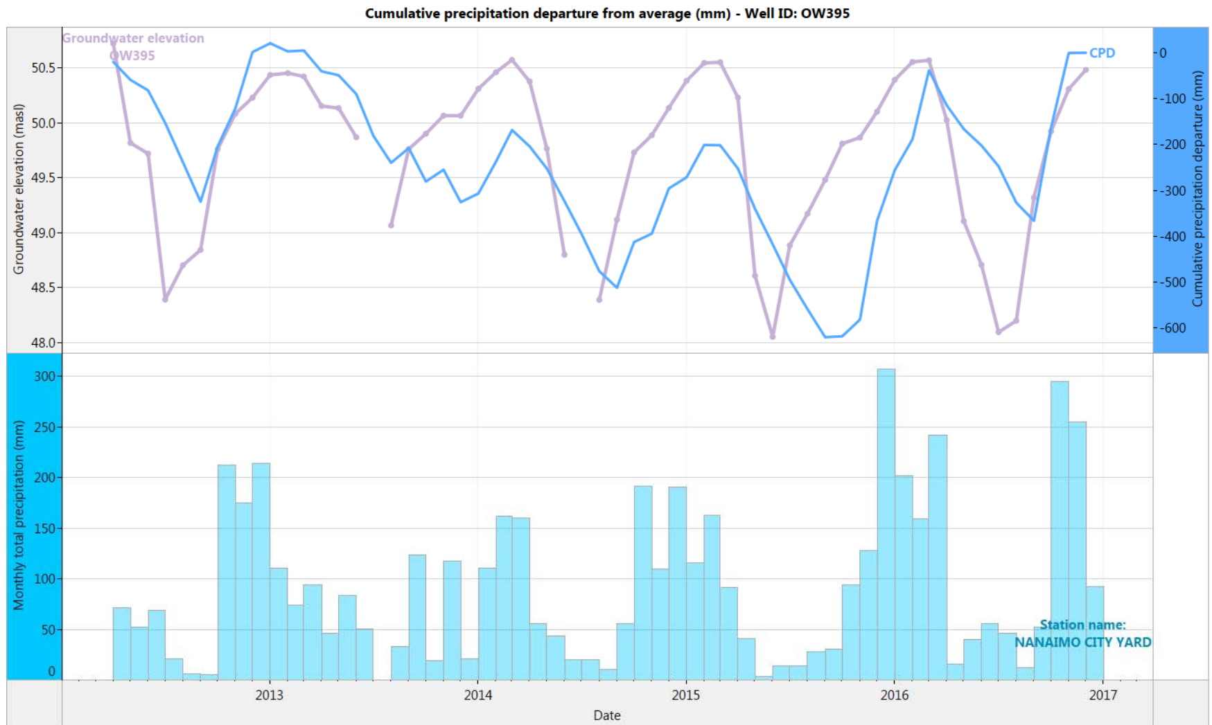
Figure 14. OW395: Month end groundwater levels compared to cumulative precipitation departure curve and total monthly precipitation (2012-2016)
