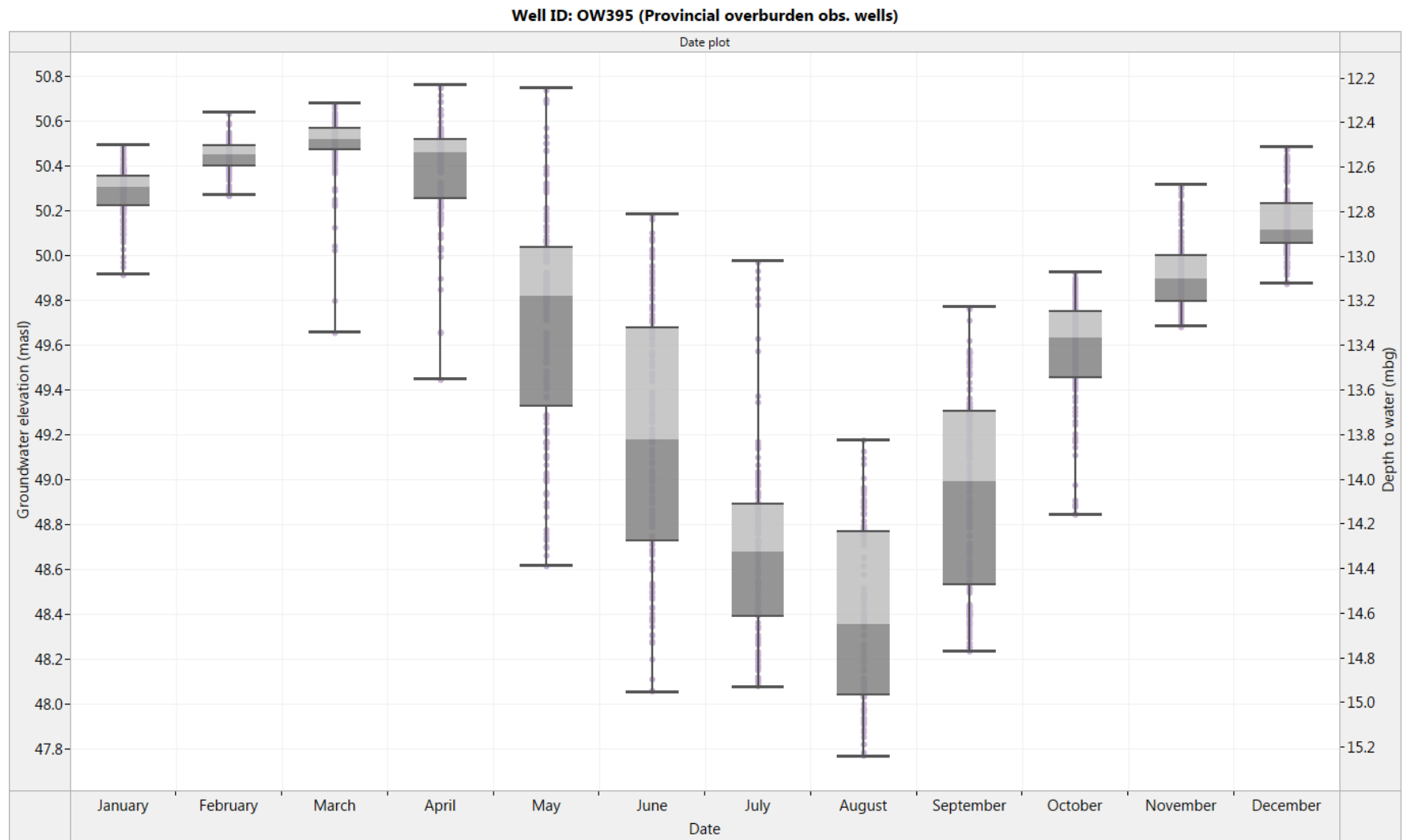
Figure 10. OW395: Box and Whisker diagram for historical monthly groundwater level fluctuation (2012-2016)
