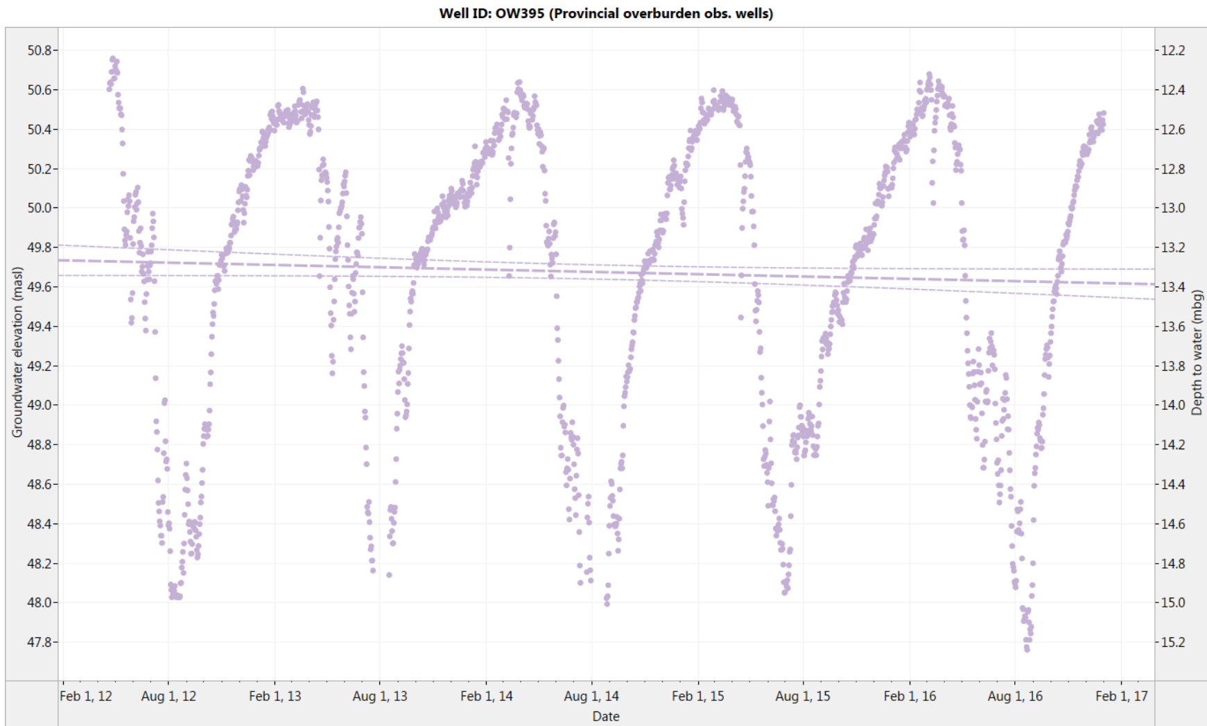
Figure 6. OW395: Historical daily water level (2012-2016) and trend line estimation (2012-2016)
