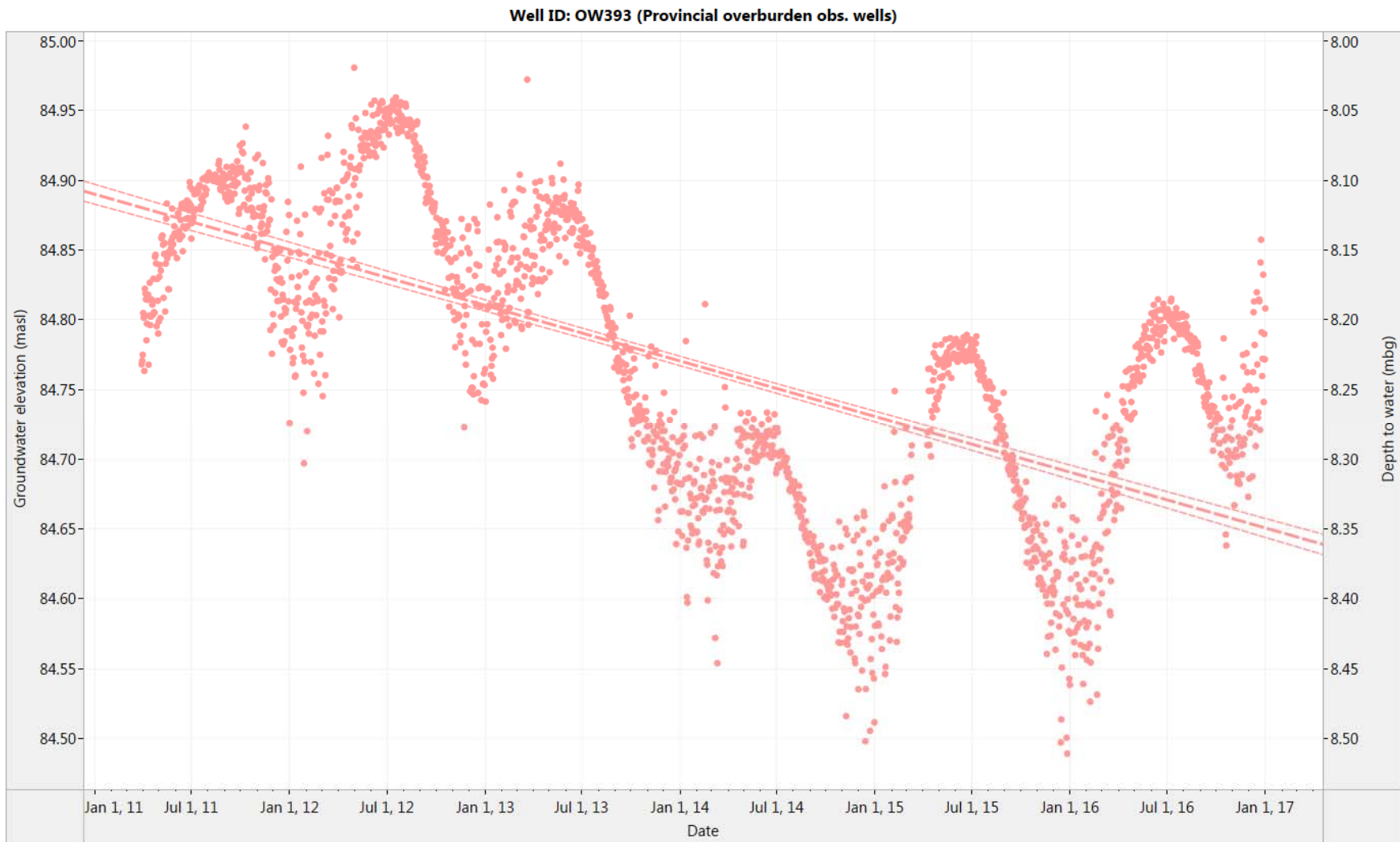
Figure 5. OW393: Historical daily water level (2011-2016) and trend line estimation (2011-2016)
