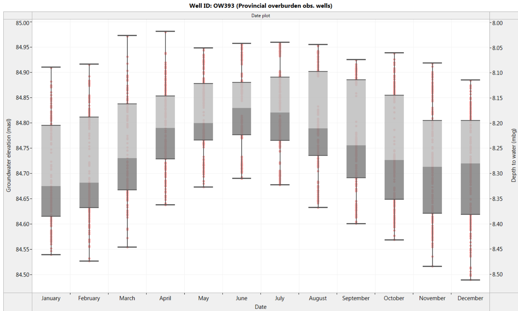
Figure 9. OW393: Box and Whisker diagram for historical monthly groundwater level fluctuation (2011-2016)
