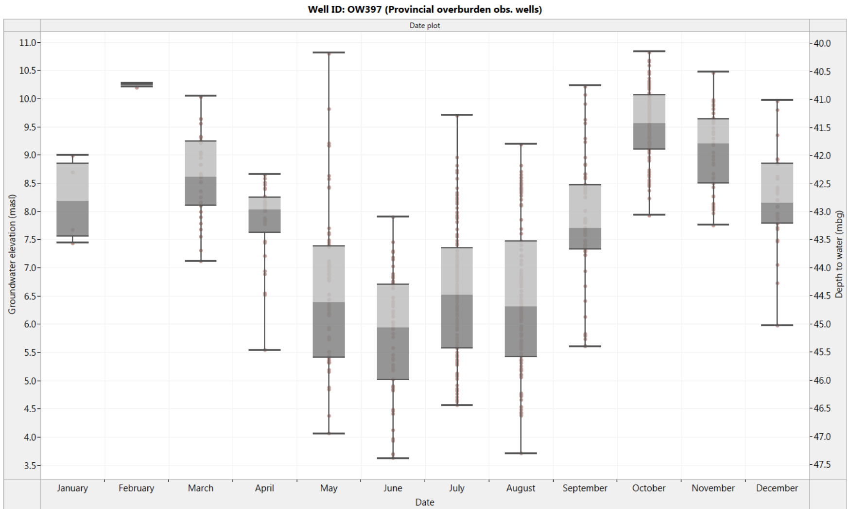
Figure 12. OW397: Box and Whisker diagram for historical monthly groundwater level fluctuation (2012-2016)
