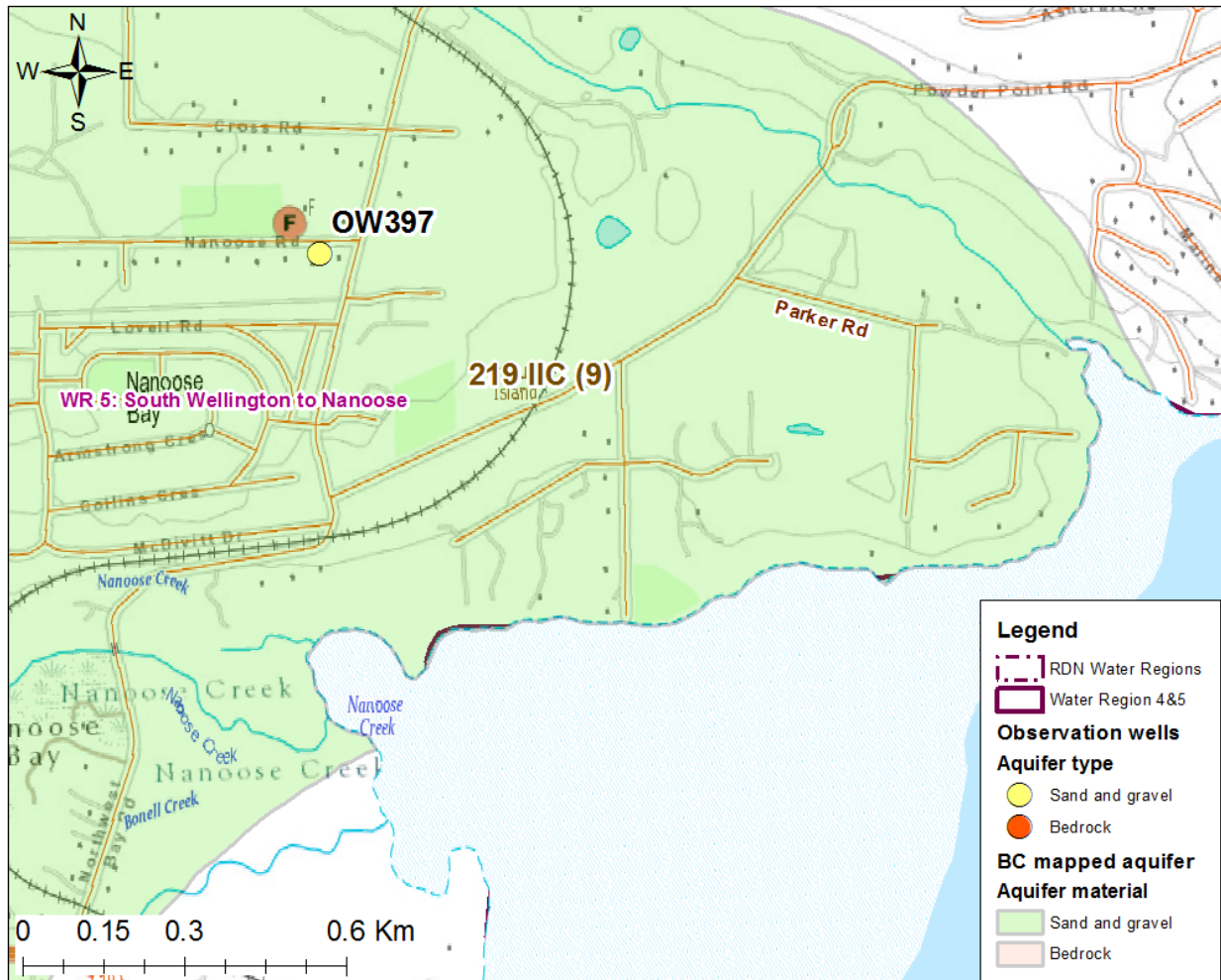
Figure 2. Location of observation well OW397
