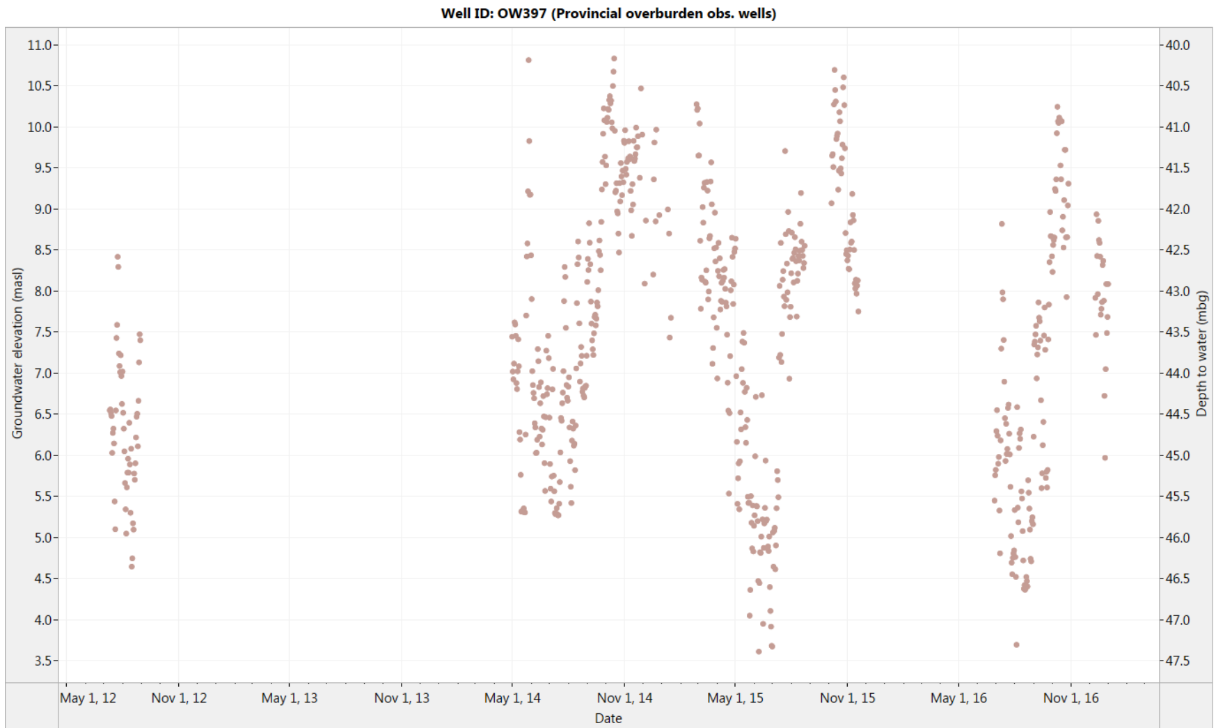
Figure 8. OW397: Historical water level (2012-2016)
