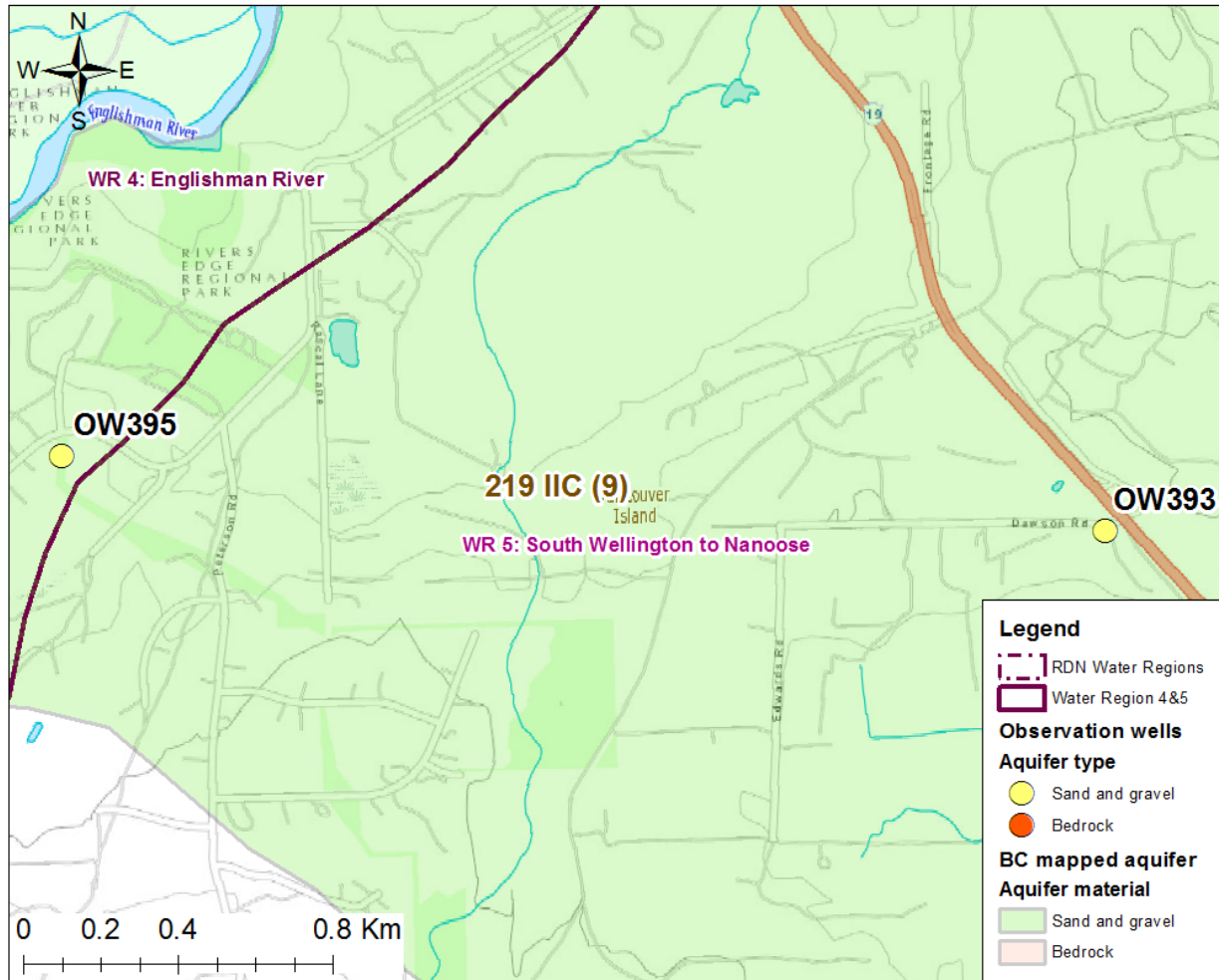
Figure 4. Location of observation wells OW393 and OW395
