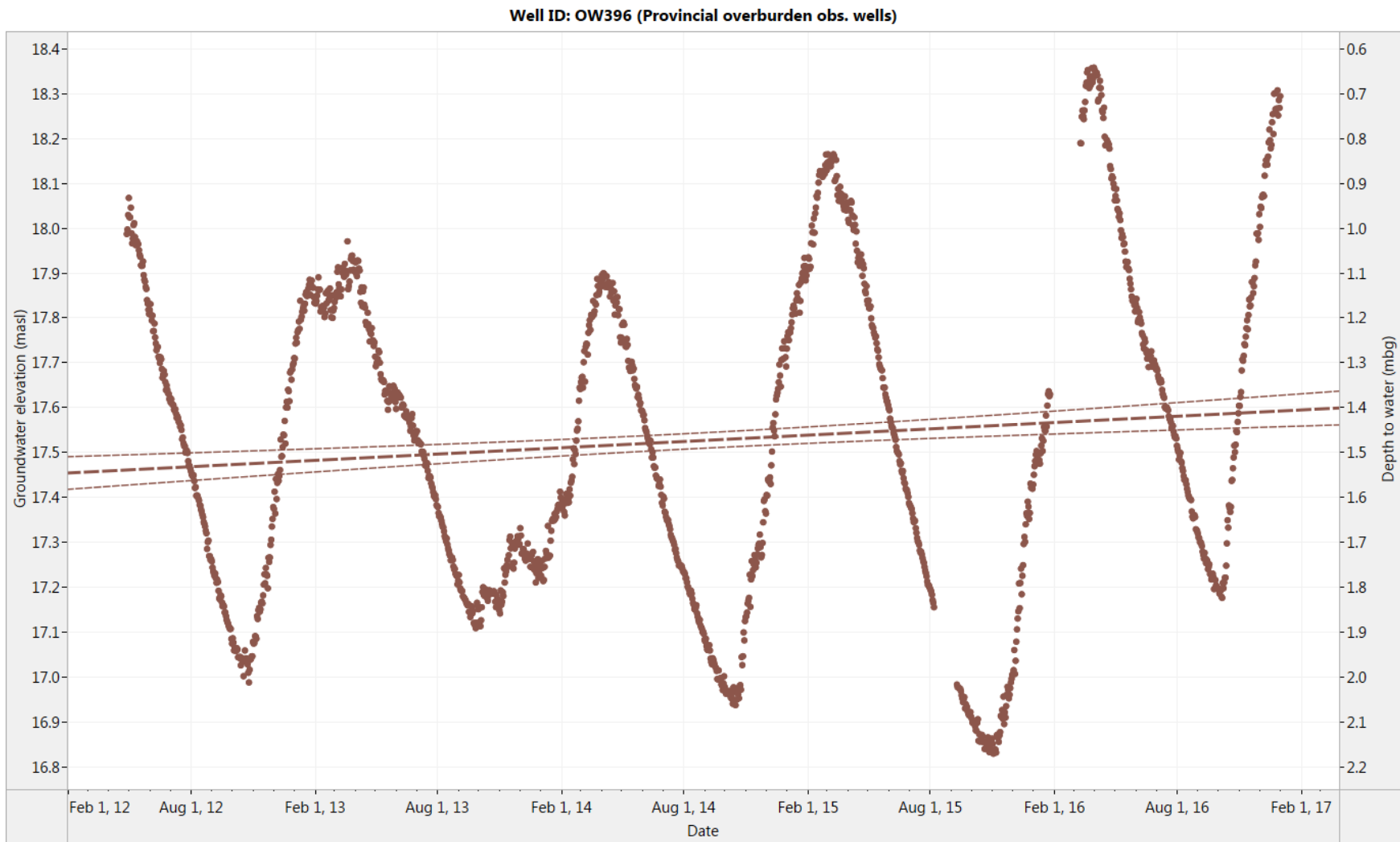
Figure 7. OW396: Historical daily water level (2012-2016) and trend line estimation (2012-2016)
