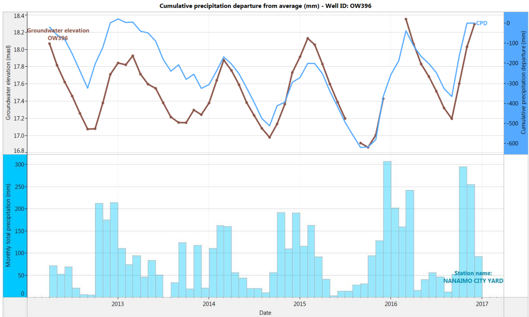
Figure 15. OW396: Month end groundwater levels compared to cumulative precipitation departure curve and total monthly precipitation (2012-2016)
