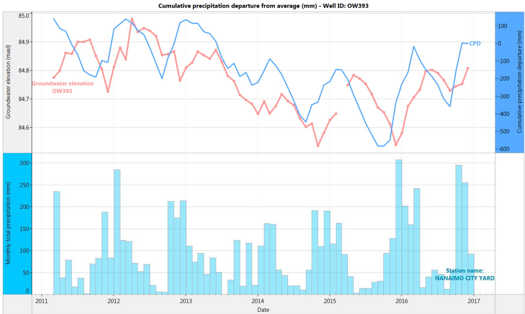
Figure 13. OW393: Month end groundwater levels compared to cumulative precipitation departure curve and total monthly precipitation (2011-2016)
